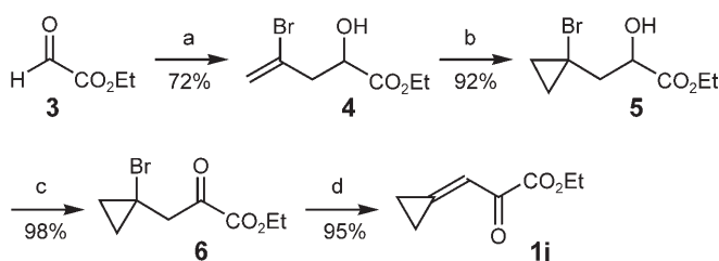
Scheme 2. Synthesis of ethyl cyclopropylidenepyruvate ( 1j ). Reagents and conditions: (a) 2,3-dibromopropene ( 2 ) (1.1 equivs.), \text{SnCl}_2 \cdot 2\text{H}_2\text{O} (1.2 equivs.), NaI, THF, 25°C, 24 h (1.2 equivs.); (b) \text{Et}_3\text{Zn} (3.3 equivs.), \text{CF}_3\text{CO}_2\text{H} (3.3 equivs.), \text{CH}_2\text{I}_2 (3.3 equivs.), \text{CH}_2\text{Cl}_2 , –5 to 0°C, 1.5 h, then 25°C, 60 h; (c) Dess–Martin periodinane (1.1 equivs.), \text{CH}_2\text{Cl}_2 , 25°C, 1 h; (d) \text{Na}_2\text{CO}_3 (5 equivs.), \text{Et}_2\text{O} , 25°C, 24 h.
