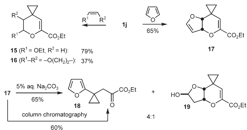
Scheme 4. Inverse electron-demand hetero-Diels-Alder reactions of ethyl cyclopropylidenepyruvate ( 1j ), and further transformations of the furan adduct of 1j . Reagents and conditions: alkene (2 mL per mmol of 1j ), neat, 25 °C, 24 h.
