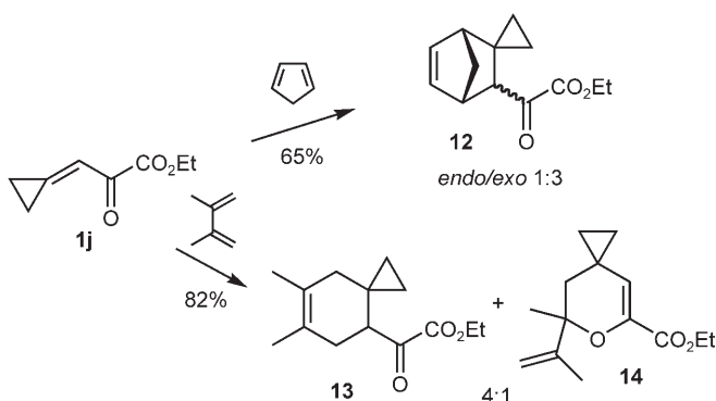
Scheme 3. Diels–Alder reactions of ethyl cyclopropylidenepyruvate ( 1j ). Reagents and conditions: diene (2 mL per mmol of 1j ) neat, 25 °C, 24 h.
